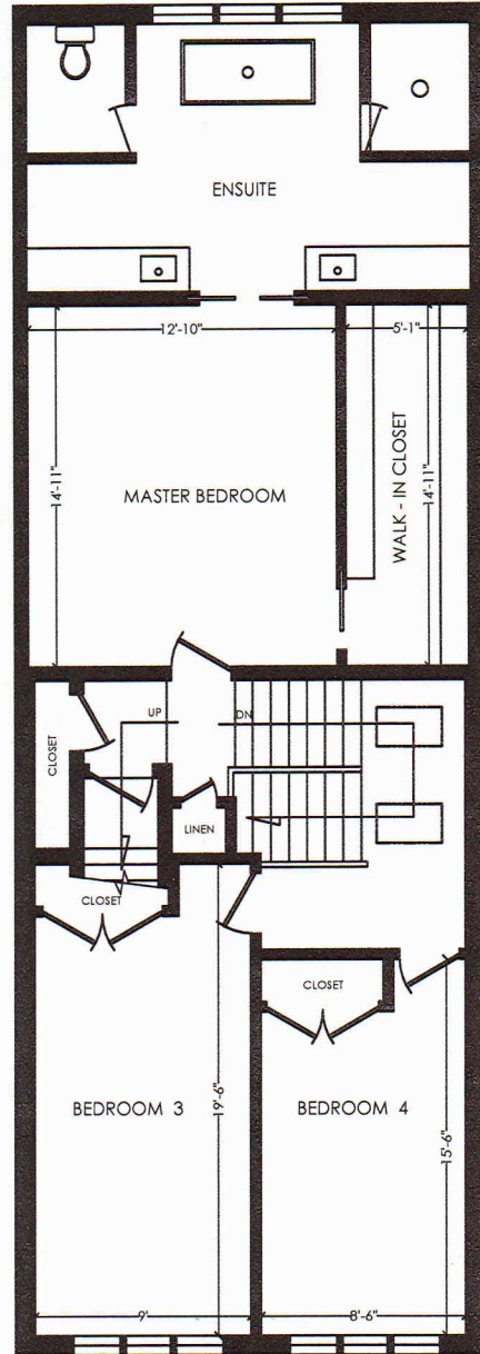
FOURTH & FIFTH FLOORS FLOOR AREA 1087 SQUARE FEET
